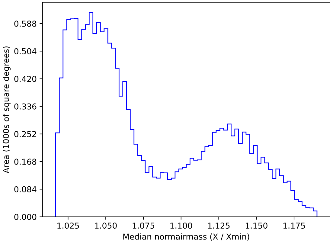
too_elab_r32_d2_giz_v3.4_10yrs WFD r band: Median normairmass
