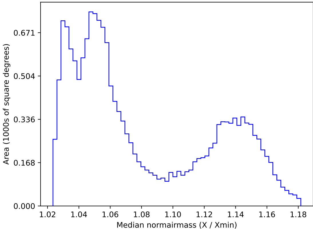
too_elab_r32_d2_giz_v3.4_10yrs WFD all bands: Median normairmass
