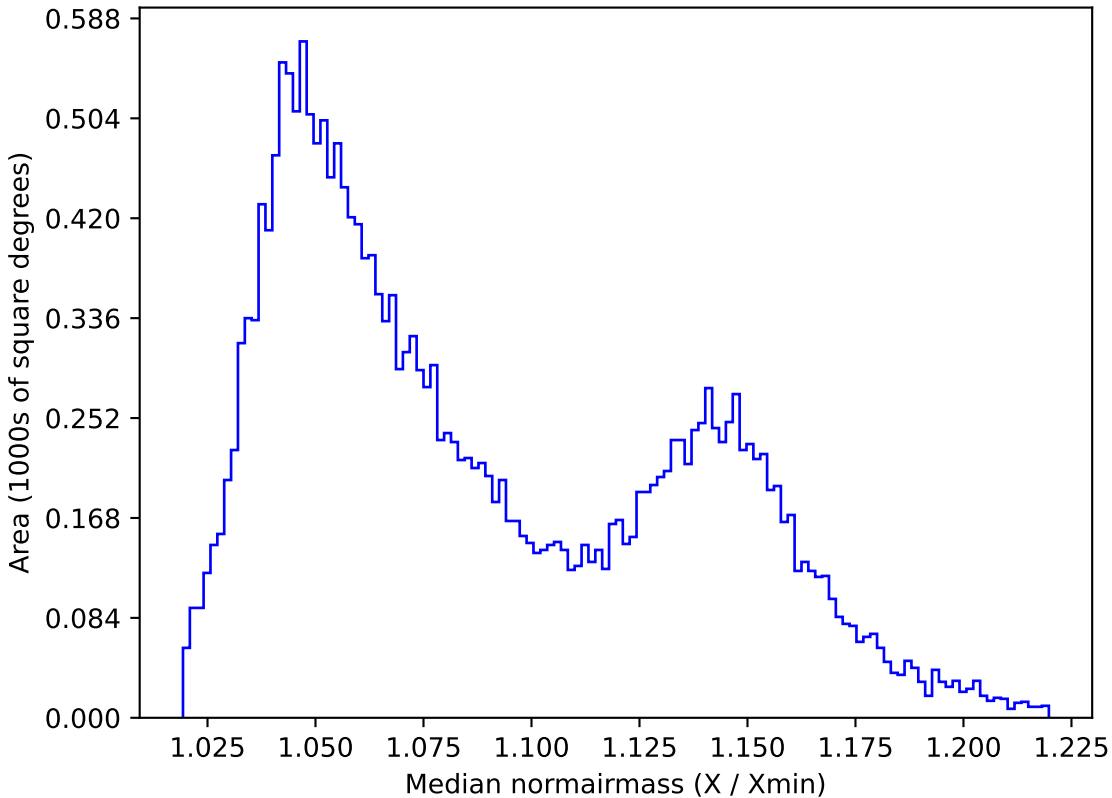
too_elab_r32_d2_giz_v3.4_10yrs All sky y band: Median normairmass
