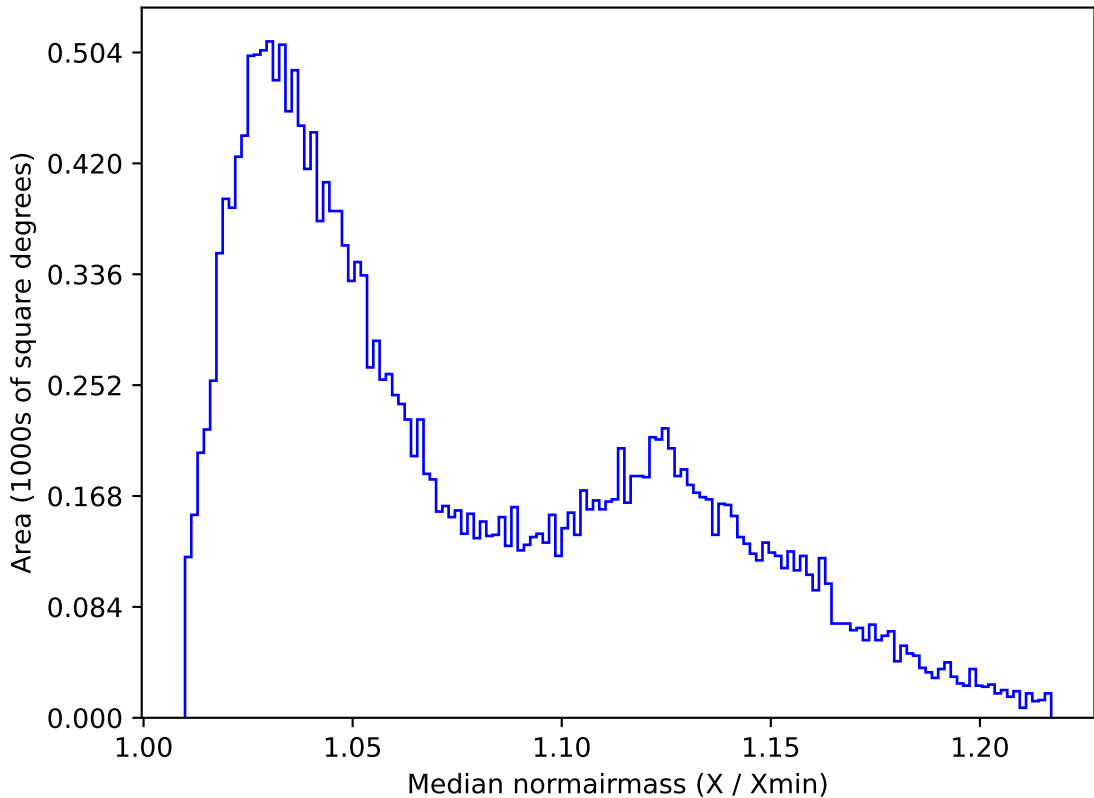
too_elab_r32_d2_giz_v3.4_10yrs All sky u band: Median normairmass
