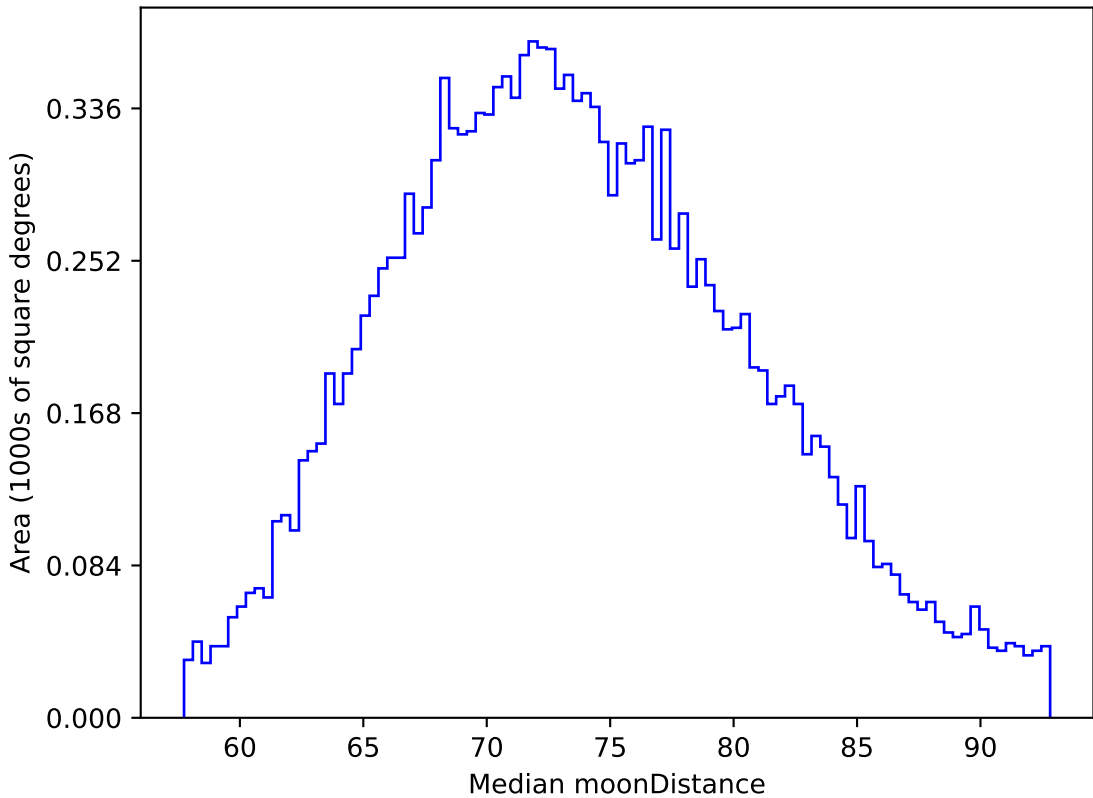
too_elab_r32_d2_giz_v3.4_10yrs WFD z band: Median moonDistance
