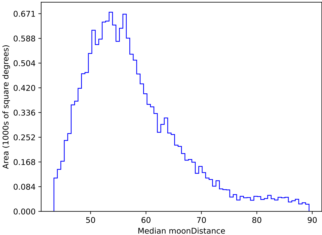
too_elab_r32_d2_giz_v3.4_10yrs WFD y band: Median moonDistance
