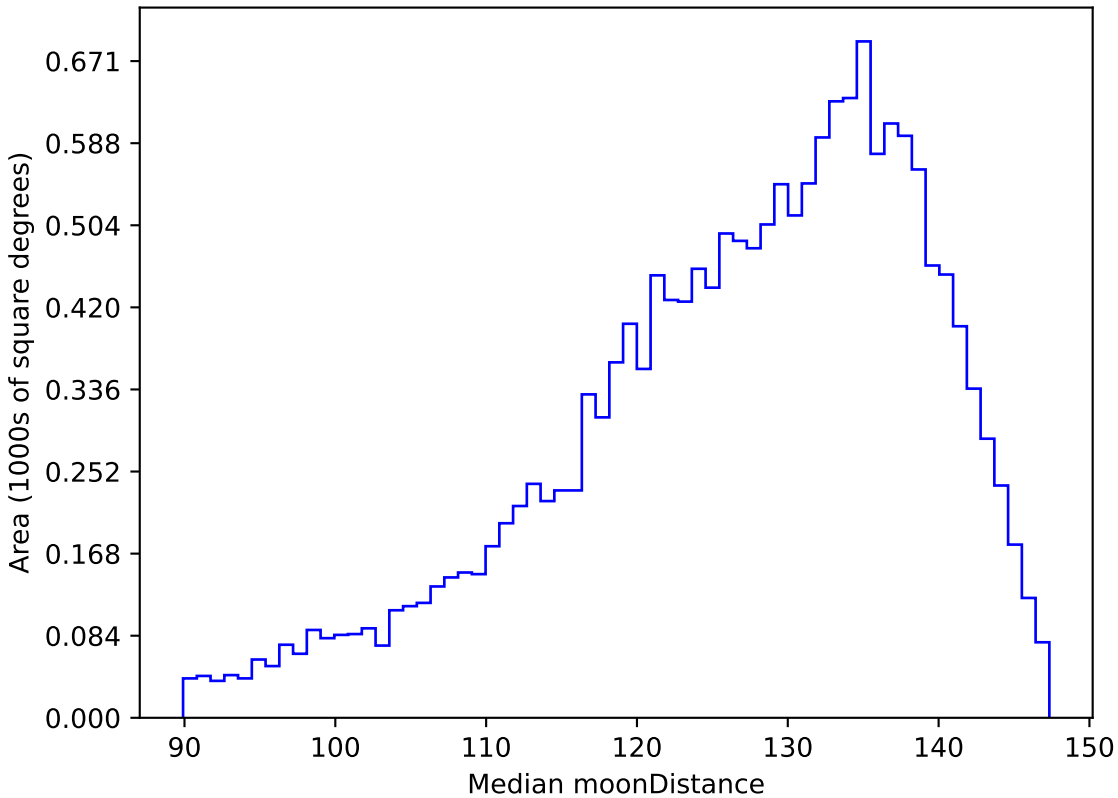
too_elab_r32_d2_giz_v3.4_10yrs WFD u band: Median moonDistance
