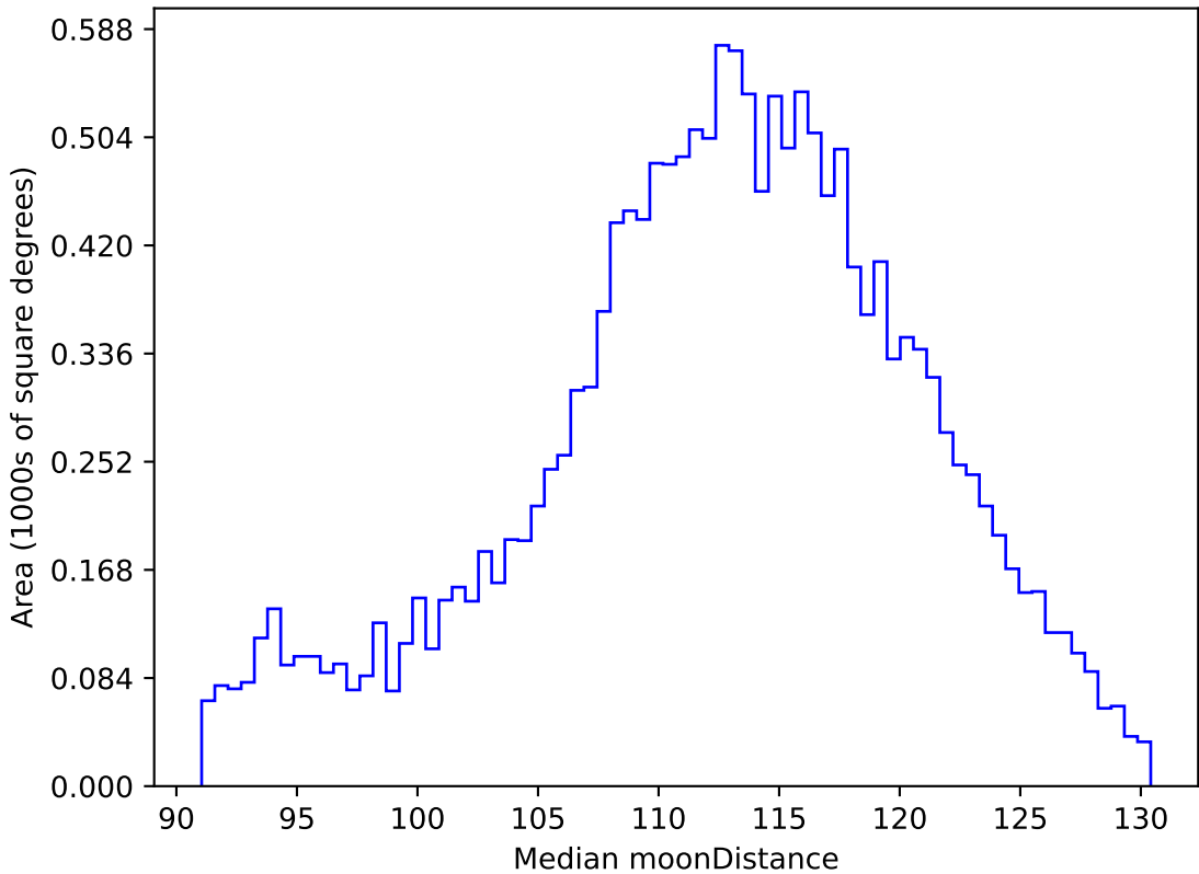
too_elab_r32_d2_giz_v3.4_10yrs WFD r band: Median moonDistance
