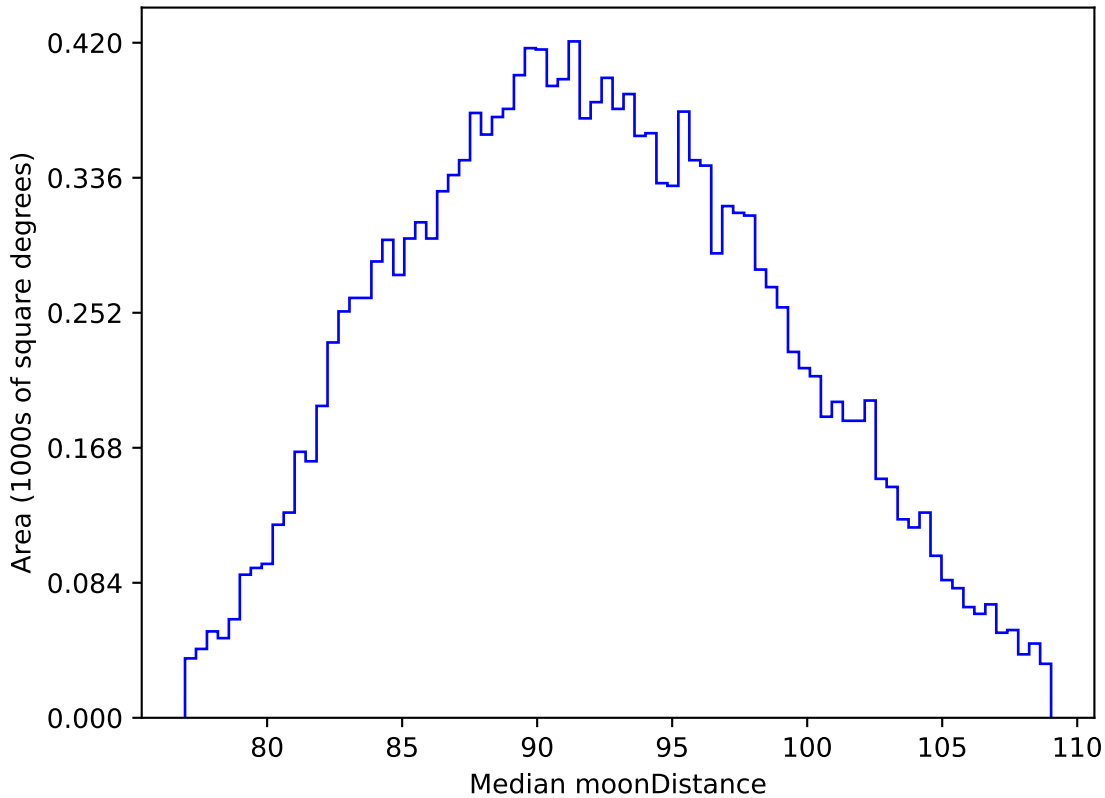
too_elab_r32_d2_giz_v3.4_10yrs WFD i band: Median moonDistance
