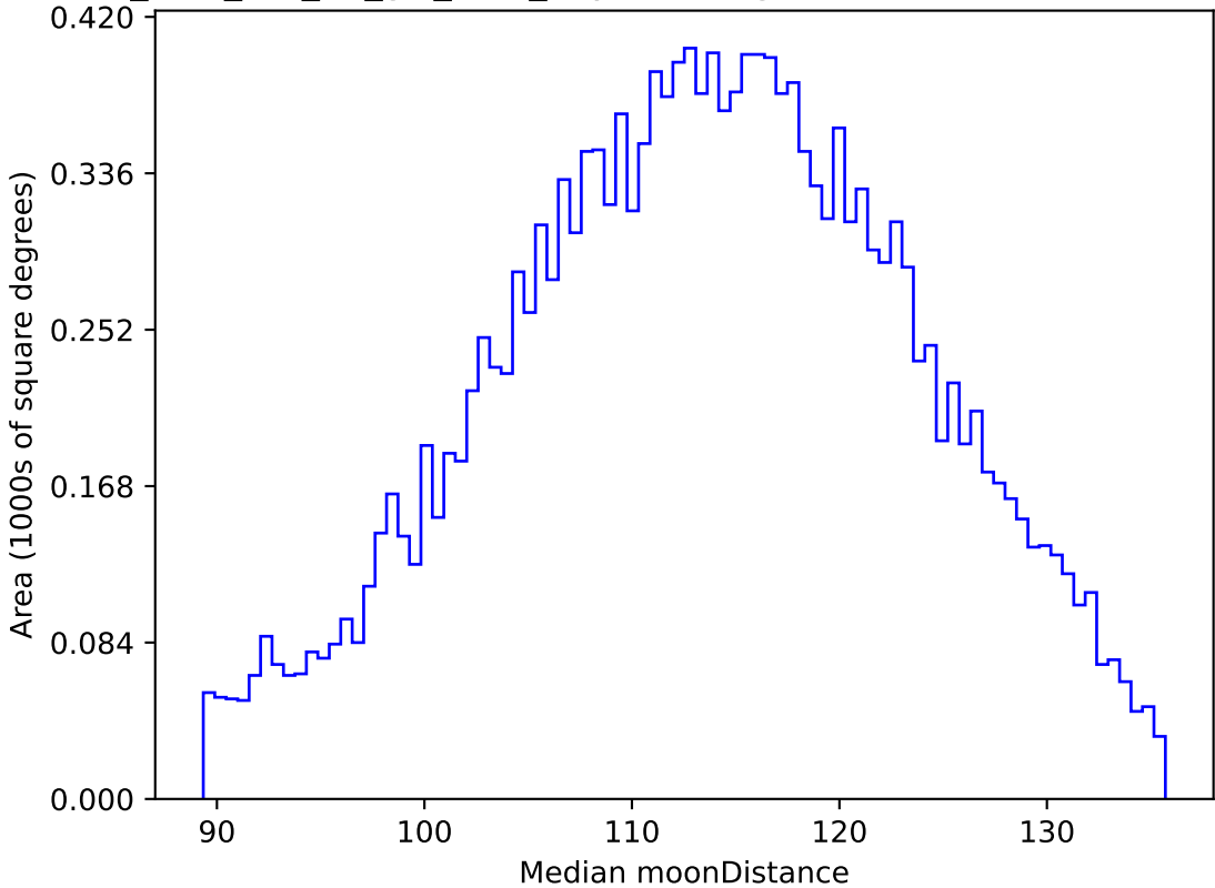
too_elab_r32_d2_giz_v3.4_10yrs WFD g band: Median moonDistance
