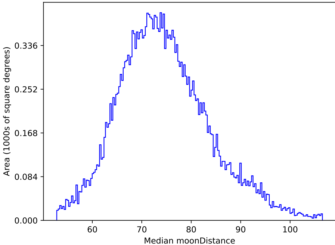
too_elab_r32_d2_giz_v3.4_10yrs All sky z band: Median moonDistance
