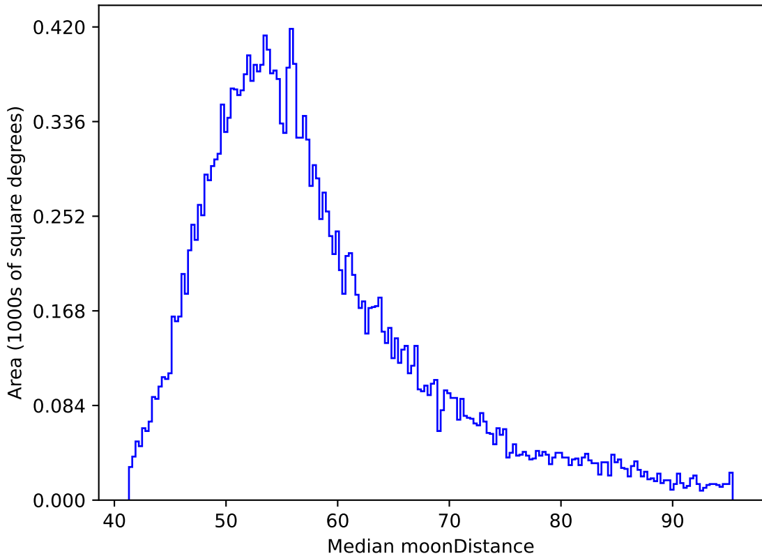
too_elab_r32_d2_giz_v3.4_10yrs All sky y band: Median moonDistance
