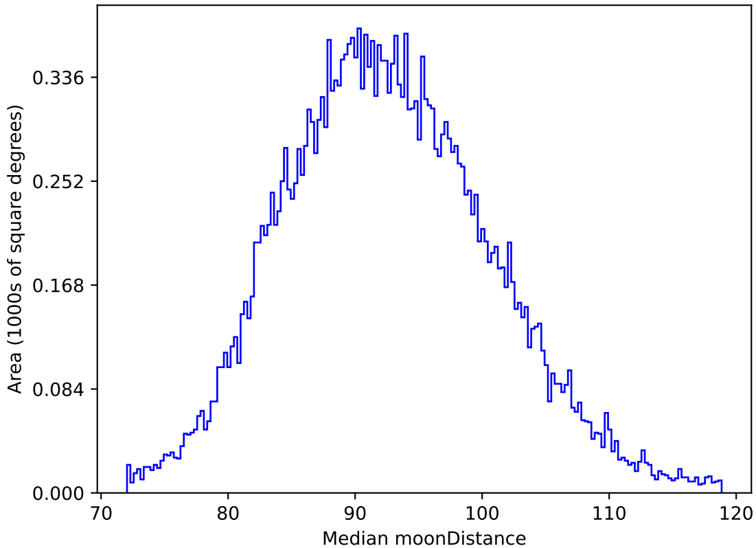
too_elab_r32_d2_giz_v3.4_10yrs All sky i band: Median moonDistance
