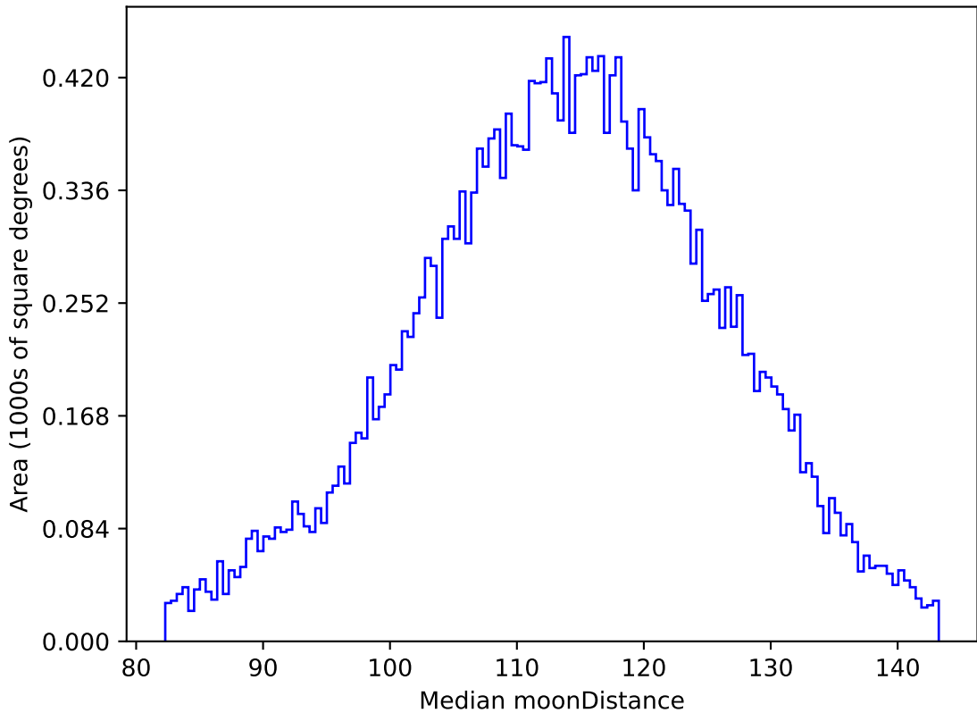
too_elab_r32_d2_giz_v3.4_10yrs All sky g band: Median moonDistance
