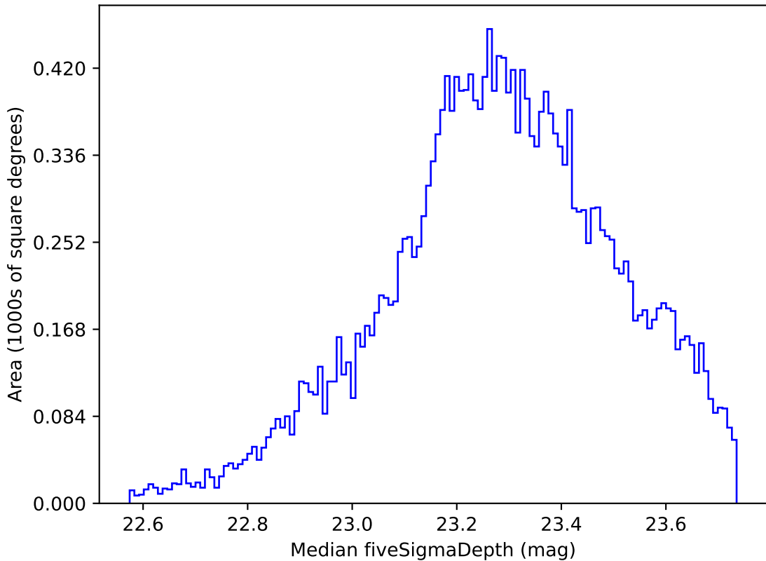
too_elab_r32_d2_giz_v3.4_10yrs Yr 1 u band: Median fiveSigmaDepth
