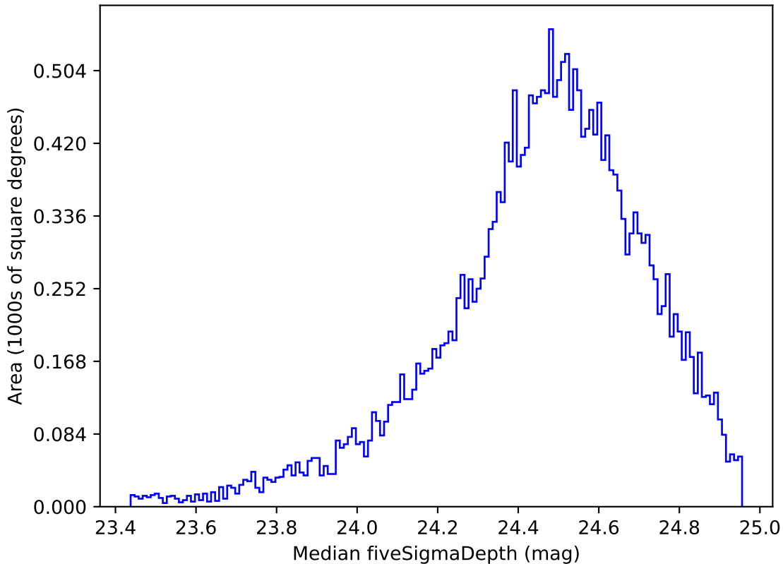
too_elab_r32_d2_giz_v3.4_10yrs Yr 1 g band: Median fiveSigmaDepth
