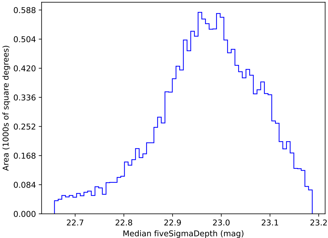
too_elab_r32_d2_giz_v3.4_10yrs WFD z band: Median fiveSigmaDepth
