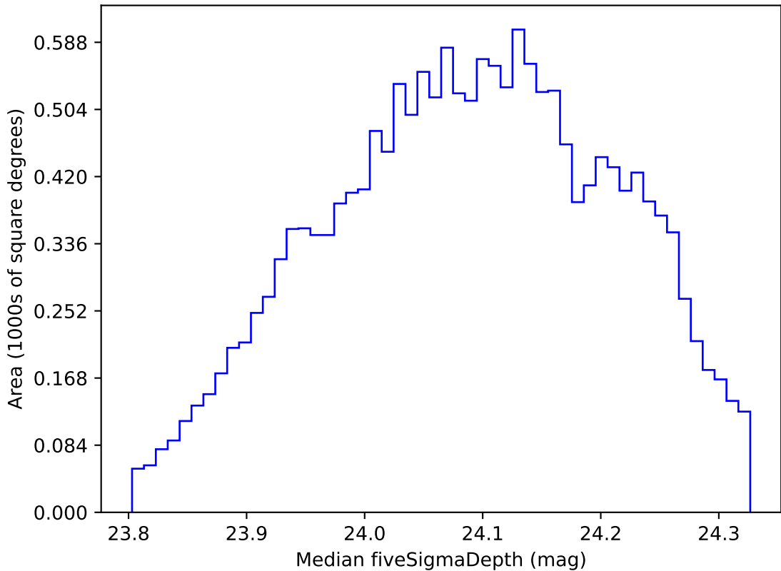
too_elab_r32_d2_giz_v3.4_10yrs WFD r band: Median fiveSigmaDepth
