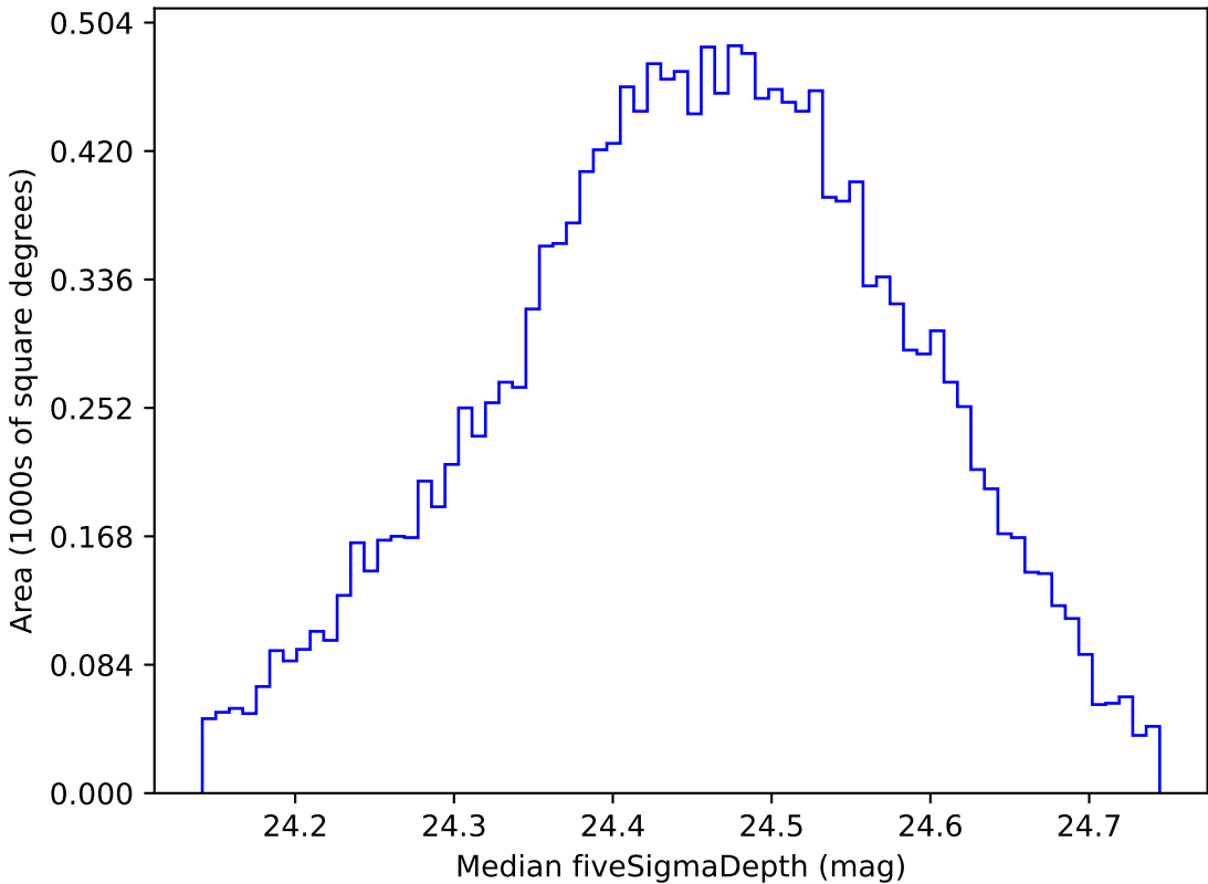
too_elab_r32_d2_giz_v3.4_10yrs WFD g band: Median fiveSigmaDepth
