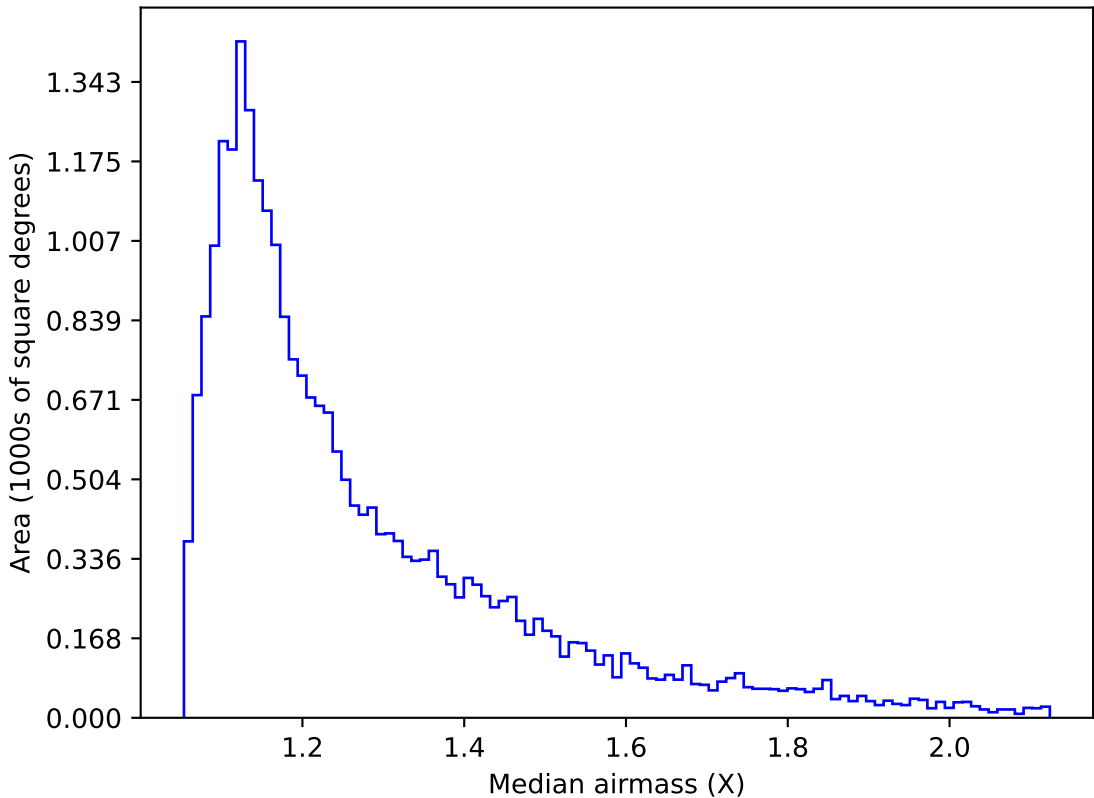
too_elab_r32_d2_giz_v3.4_10yrs Yr 1 g band: Median airmass
