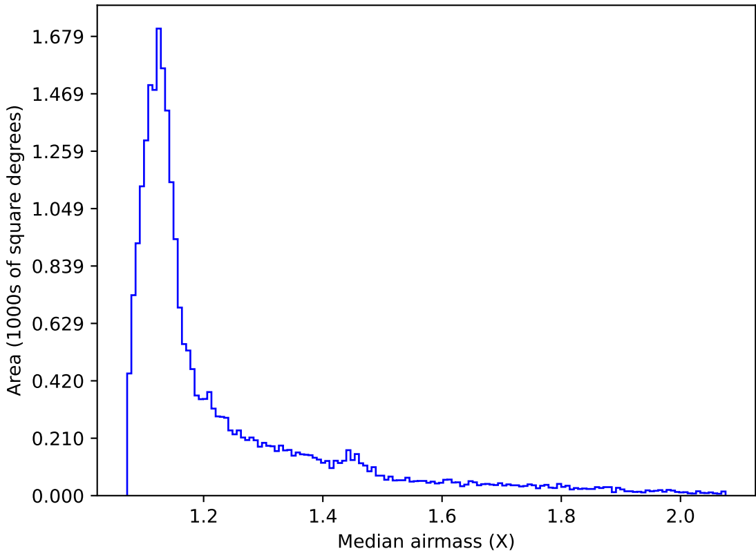
too_elab_r32_d2_giz_v3.4_10yrs Yr 1 all bands: Median airmass
