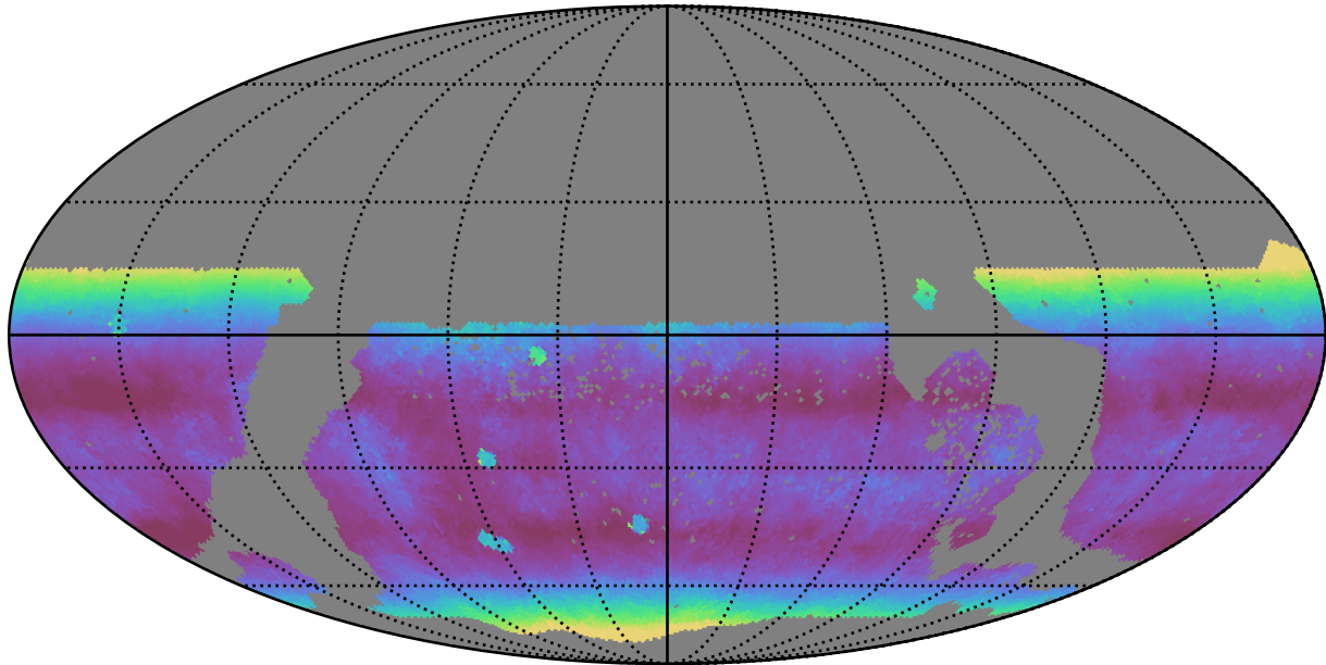
too_elab_r32_d2_giz_v3.4_10yrs WFD z band: Median airmass
