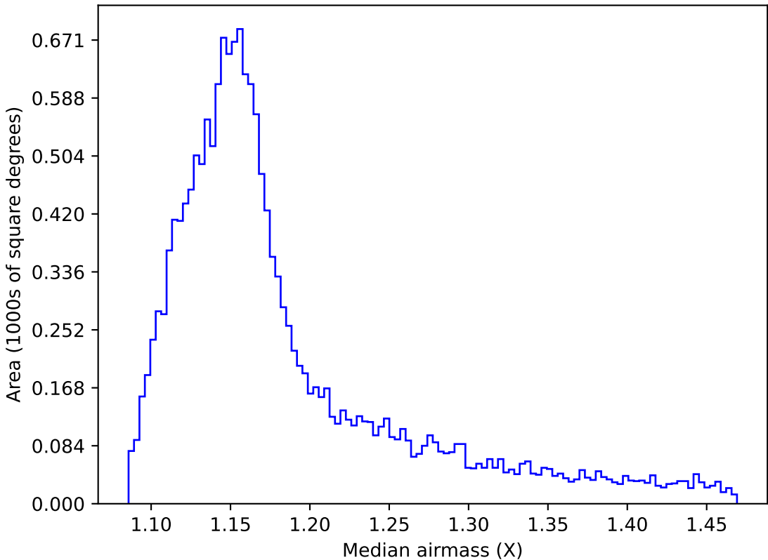
too_elab_r32_d2_giz_v3.4_10yrs WFD z band: Median airmass
