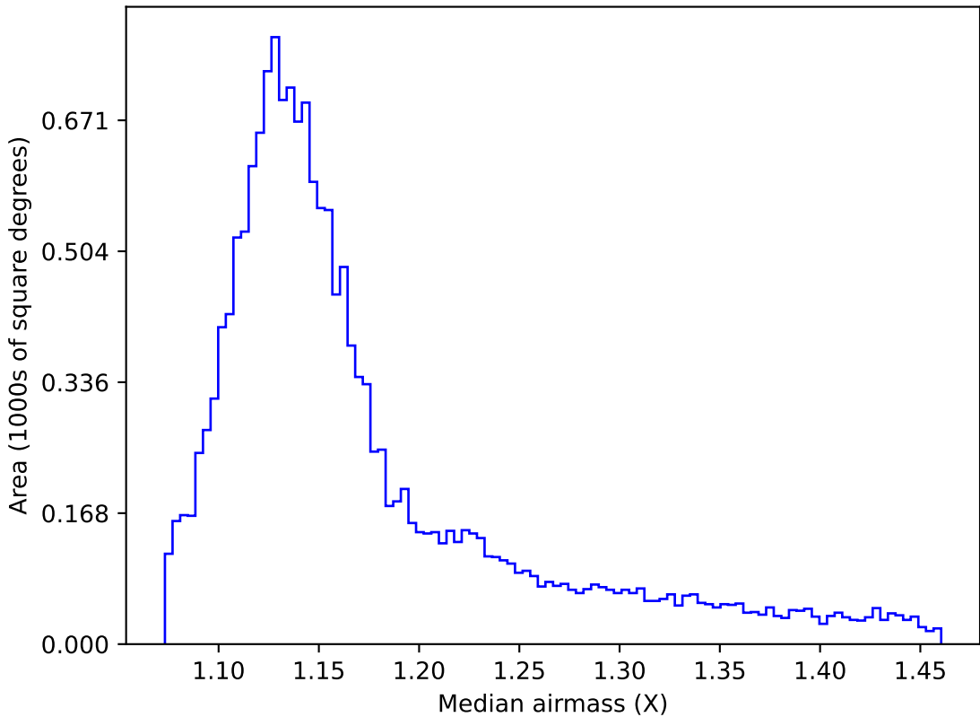
too_elab_r32_d2_giz_v3.4_10yrs WFD r band: Median airmass
