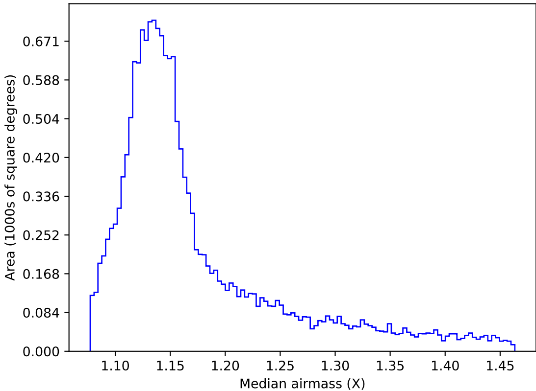
too_elab_r32_d2_giz_v3.4_10yrs WFD i band: Median airmass
