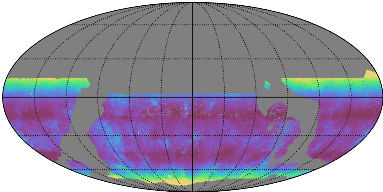
too_elab_r32_d2_giz_v3.4_10yrs WFD g band: Median airmass
