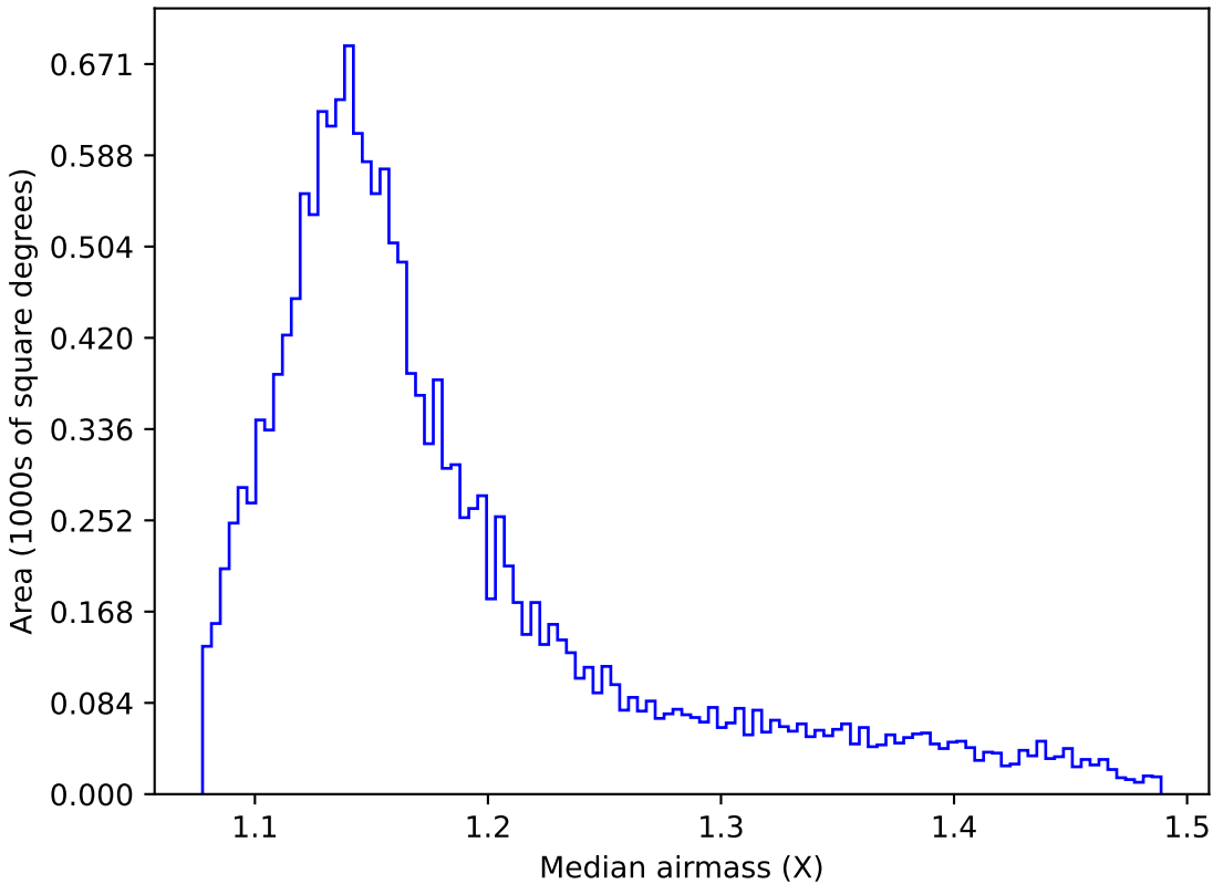
too_elab_r32_d2_giz_v3.4_10yrs WFD g band: Median airmass
