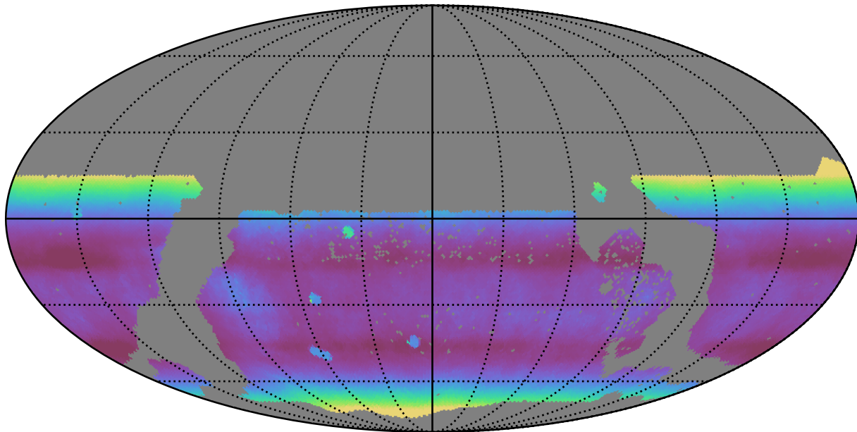
too_elab_r32_d2_giz_v3.4_10yrs WFD all bands: Median airmass
