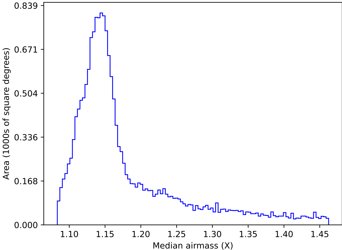
too_elab_r32_d2_giz_v3.4_10yrs WFD all bands: Median airmass
