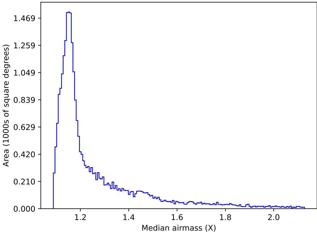
too_elab_r32_d2_giz_v3.4_10yrs All sky z band: Median airmass
