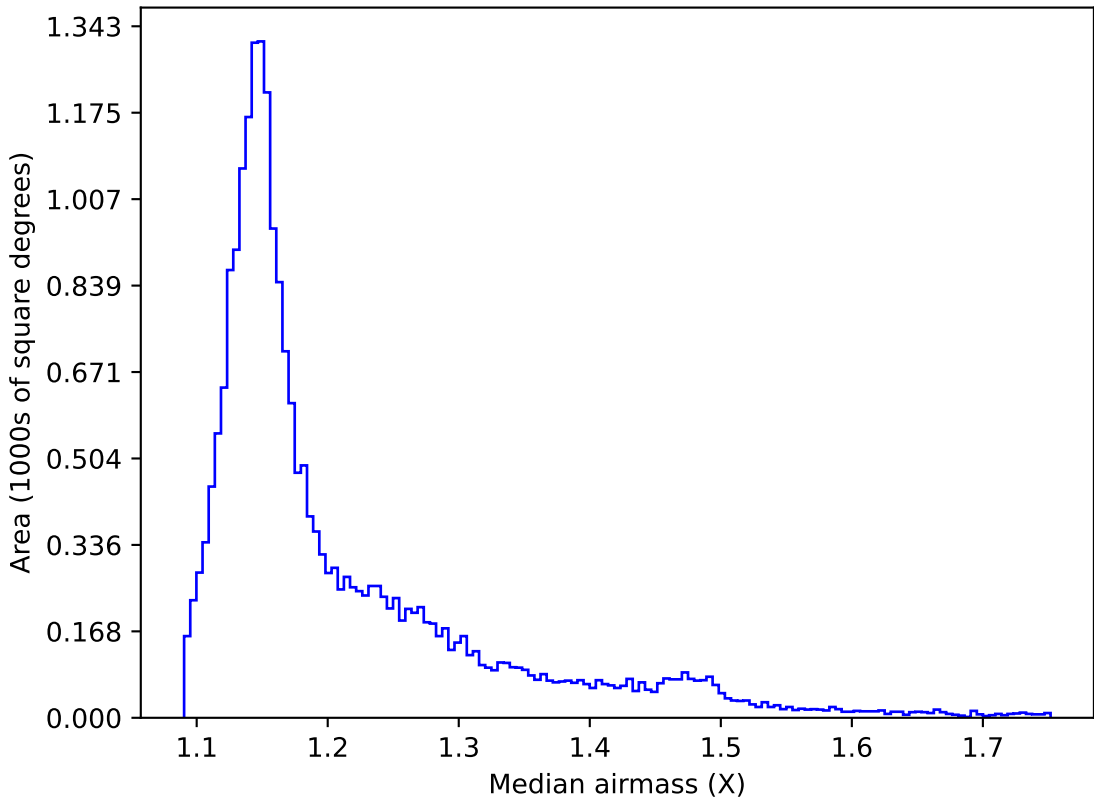
too_elab_r32_d2_giz_v3.4_10yrs All sky y band: Median airmass
