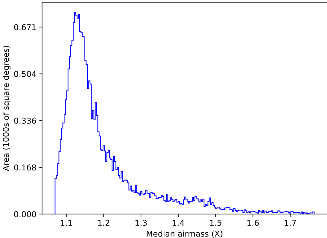
too_elab_r32_d2_giz_v3.4_10yrs All sky u band: Median airmass
