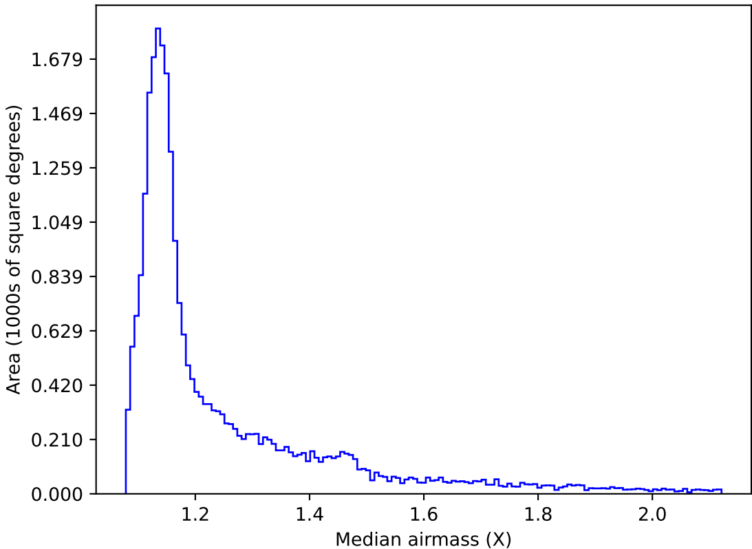
too_elab_r32_d2_giz_v3.4_10yrs All sky i band: Median airmass
