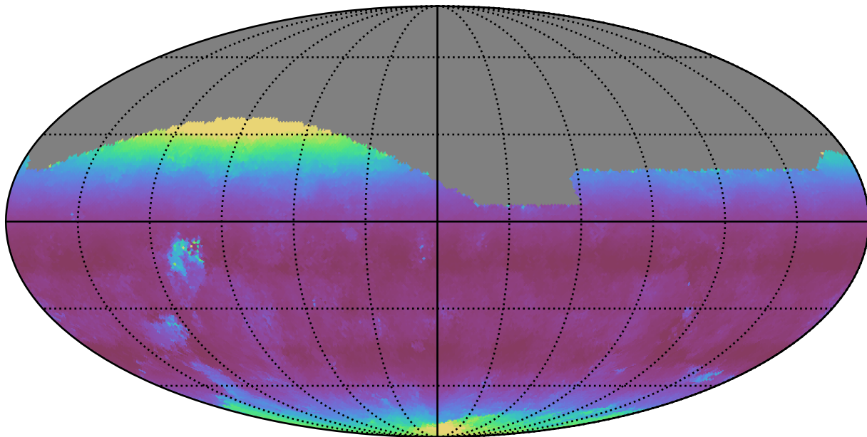
too_elab_r32_d2_giz_v3.4_10yrs All sky g band: Median airmass
