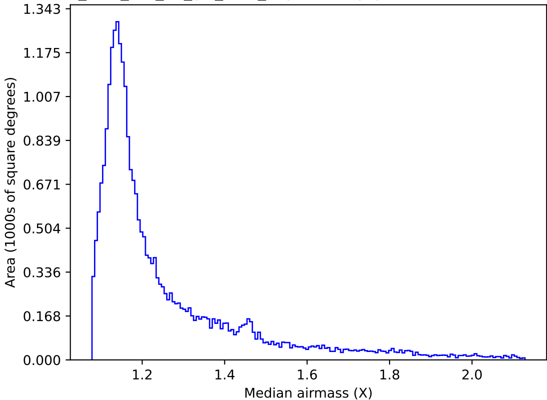
too_elab_r32_d2_giz_v3.4_10yrs All sky g band: Median airmass
