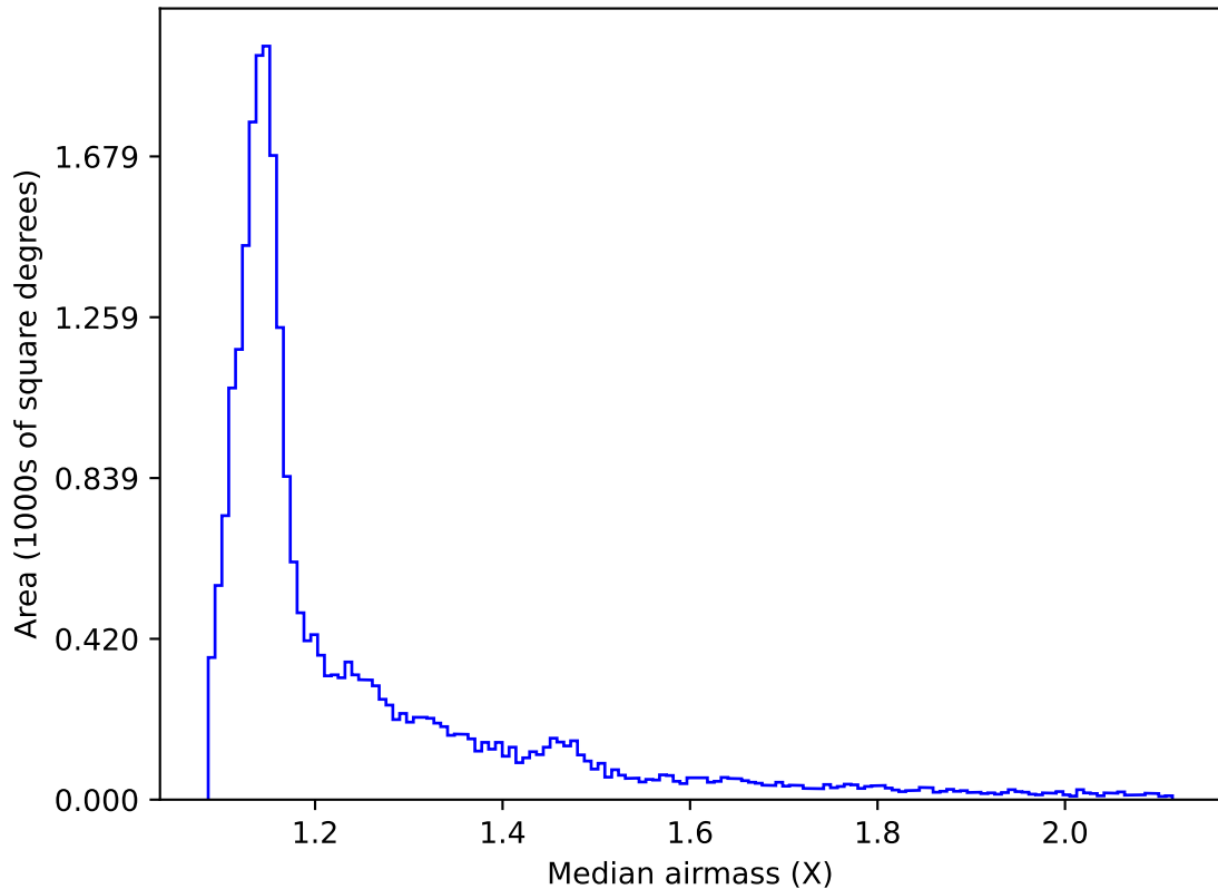
too_elab_r32_d2_giz_v3.4_10yrs All sky all bands: Median airmass
