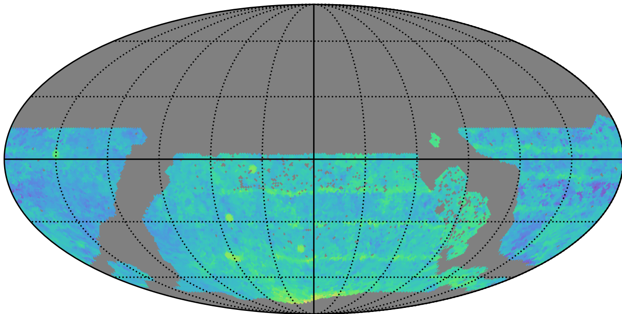
too_elab_r32_d2_giz_v3.4_10yrs WFD z band: Median Season Length
