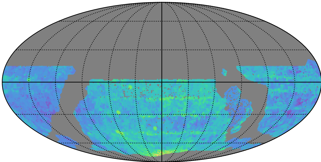
too_elab_r32_d2_giz_v3.4_10yrs WFD y band: Median Season Length
