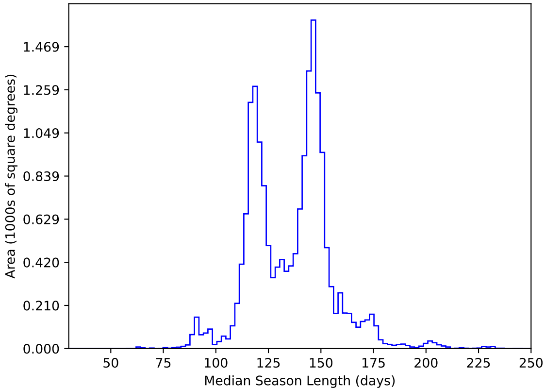
too_elab_r32_d2_giz_v3.4_10yrs WFD y band: Median Season Length
