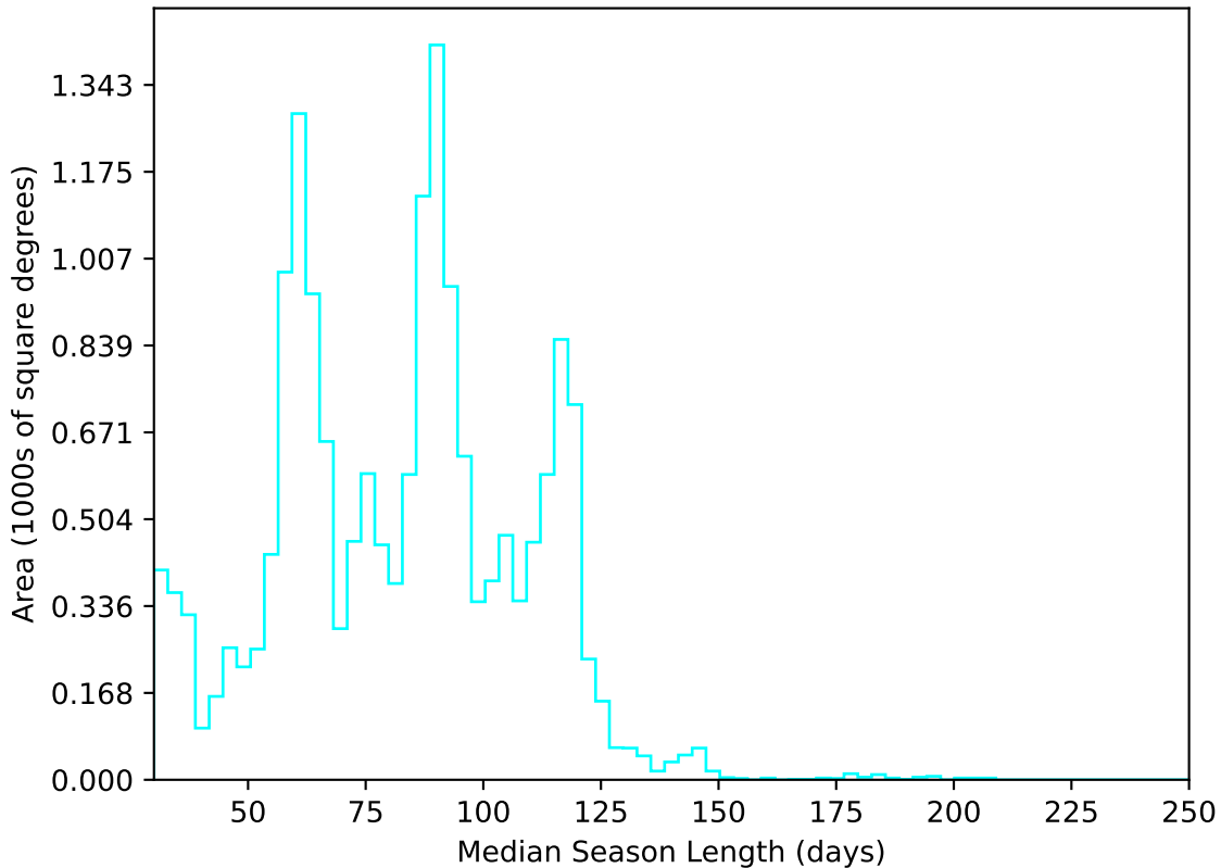
too_elab_r32_d2_giz_v3.4_10yrs WFD u band: Median Season Length
