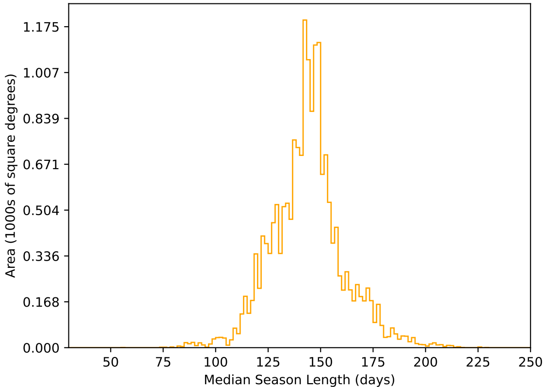
too_elab_r32_d2_giz_v3.4_10yrs WFD r band: Median Season Length
