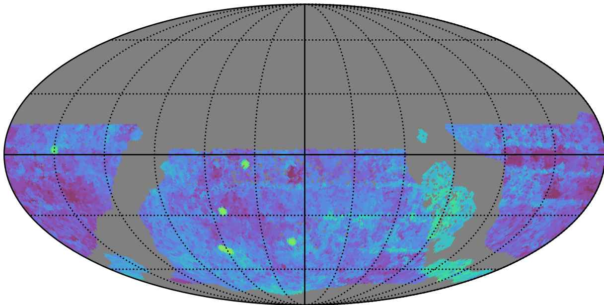
too_elab_r32_d2_giz_v3.4_10yrs WFD g band: Median Season Length
