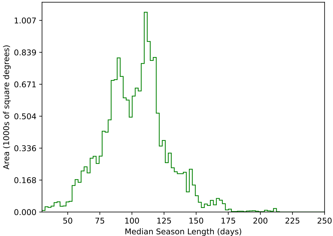
too_elab_r32_d2_giz_v3.4_10yrs WFD g band: Median Season Length
