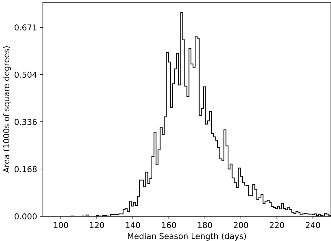
too_elab_r32_d2_giz_v3.4_10yrs WFD all bands: Median Season Length
