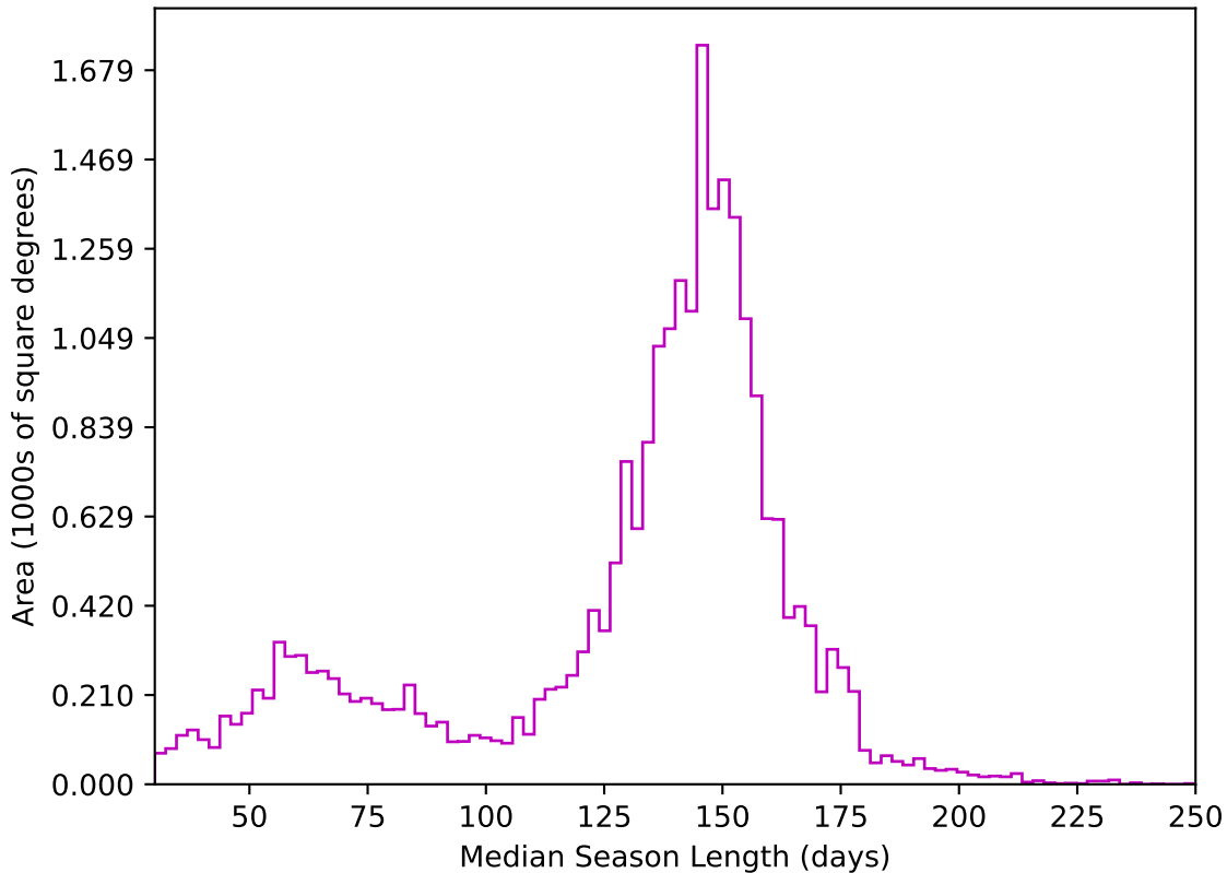
too_elab_r32_d2_giz_v3.4_10yrs All sky z band: Median Season Length
