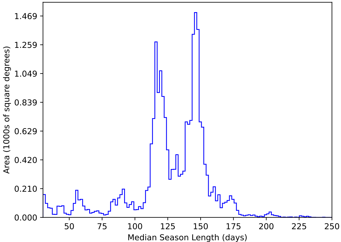
too_elab_r32_d2_giz_v3.4_10yrs All sky y band: Median Season Length
