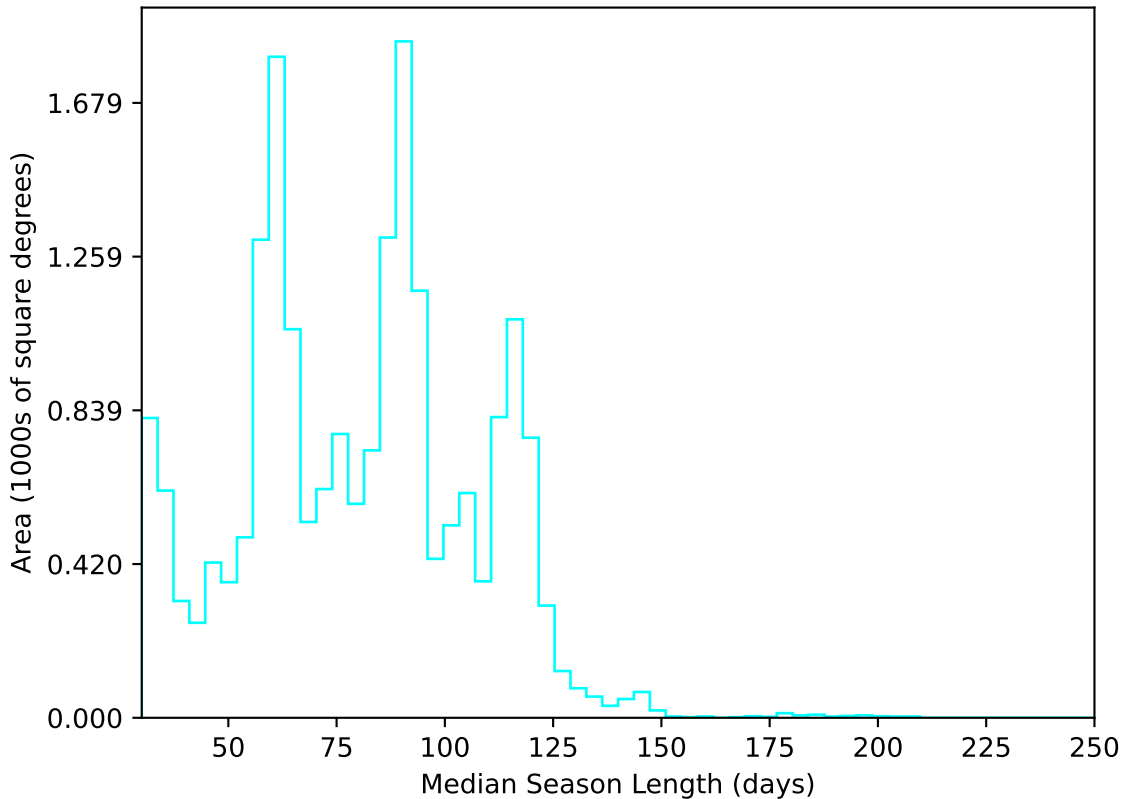
too_elab_r32_d2_giz_v3.4_10yrs All sky u band: Median Season Length
