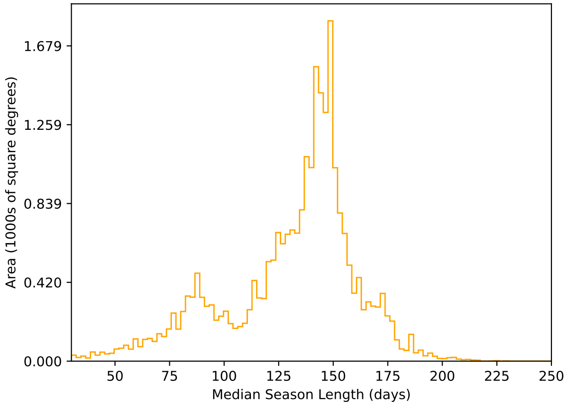
too_elab_r32_d2_giz_v3.4_10yrs All sky r band: Median Season Length
