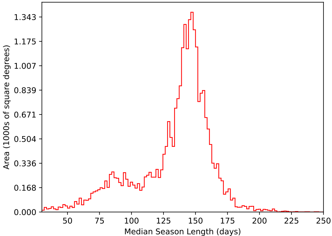
too_elab_r32_d2_giz_v3.4_10yrs All sky i band: Median Season Length
