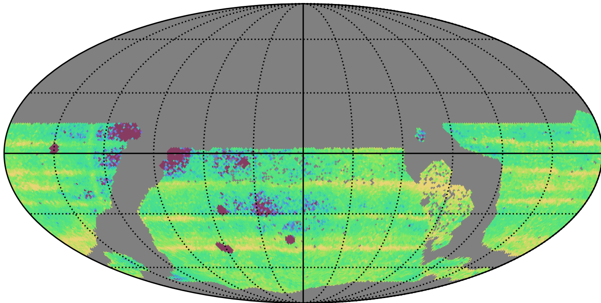
too_elab_r32_d2_giz_v3.4_10yrs WFD: Median Intra-Night Gap
